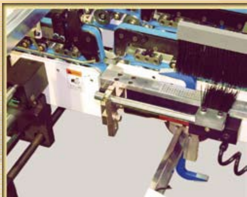
四角裝置 4-Corner Back Finger Attachment
